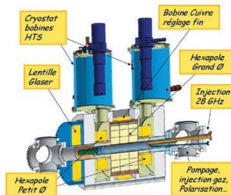
Figure 14: Conception de la source A-PHOENIX.
