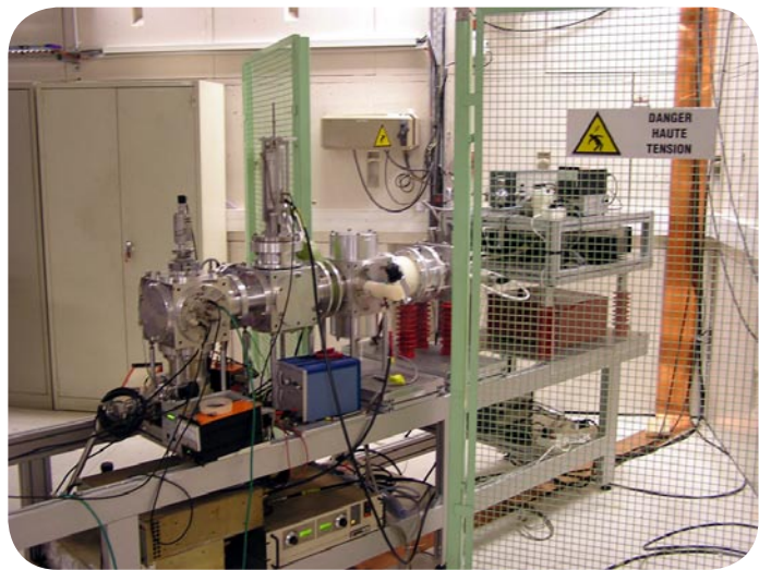
Figure 19: Banc MIMAC-He3.
